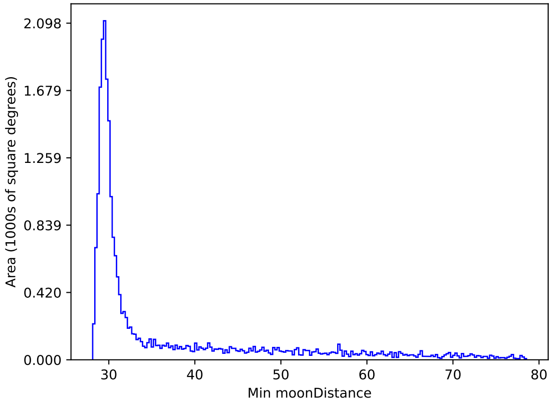
roll_pause_mjdp270_v3.4_10yrs All sky y band: Min moonDistance
