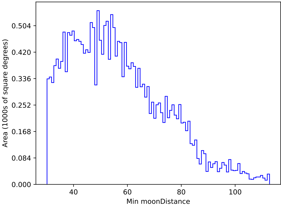
roll_pause_mjdp270_v3.4_10yrs All sky u band: Min moonDistance
