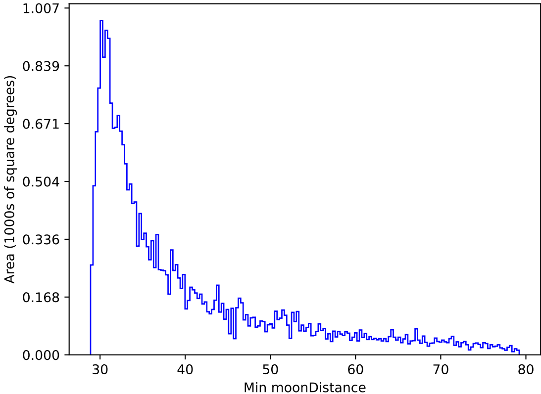
roll_pause_mjdp270_v3.4_10yrs All sky r band: Min moonDistance
