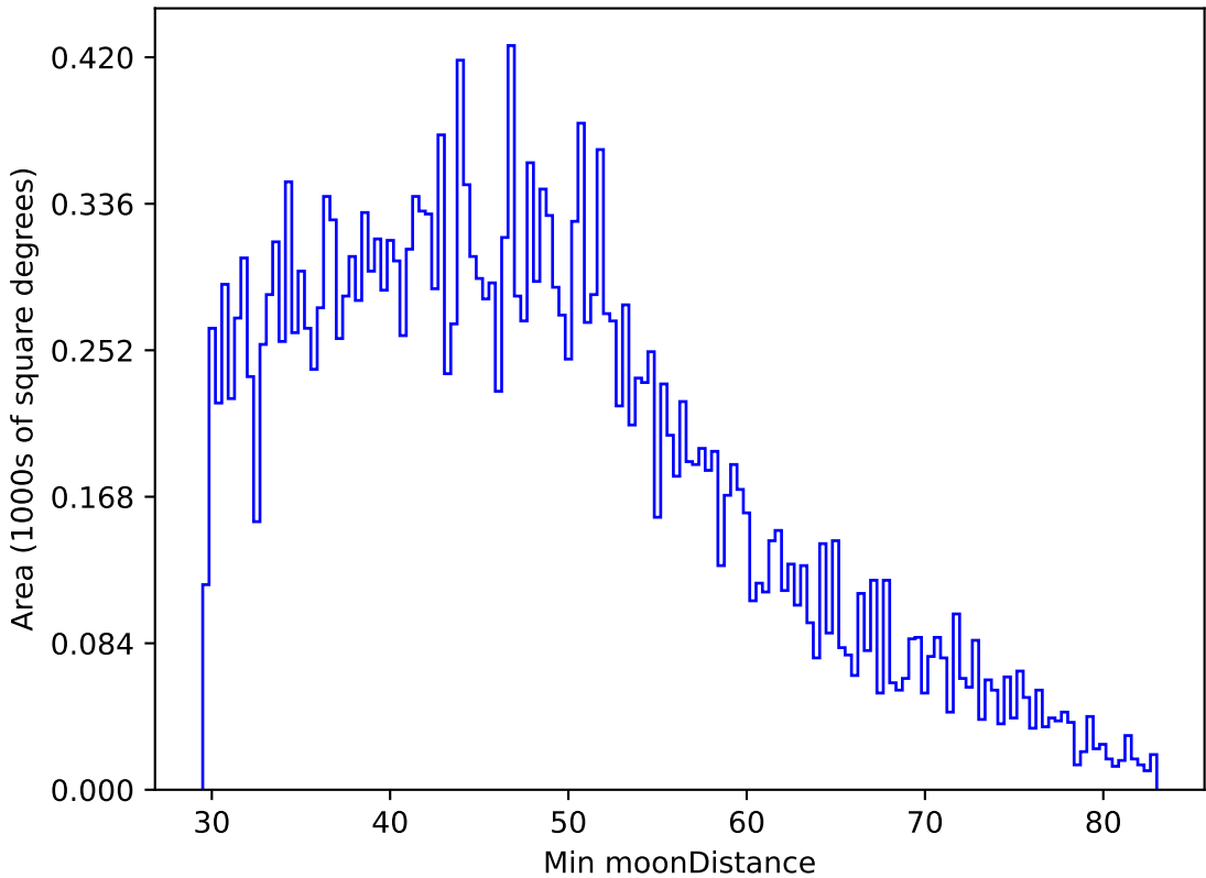
roll_pause_mjdp270_v3.4_10yrs All sky g band: Min moonDistance
