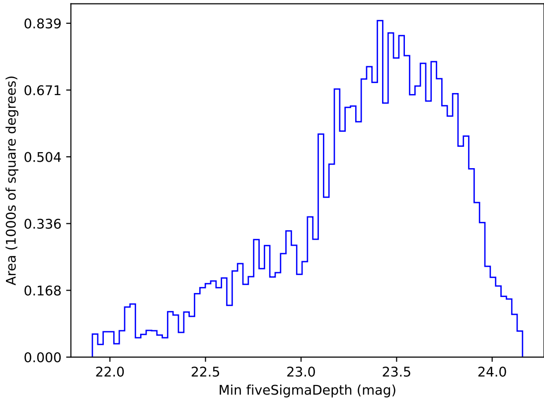
roll_pause_mjdp270_v3.4_10yrs Yr 1 r band: Min fiveSigmaDepth
