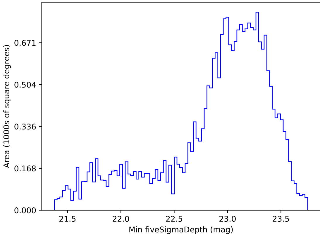
roll_pause_mjdp270_v3.4_10yrs Yr 1 i band: Min fiveSigmaDepth
