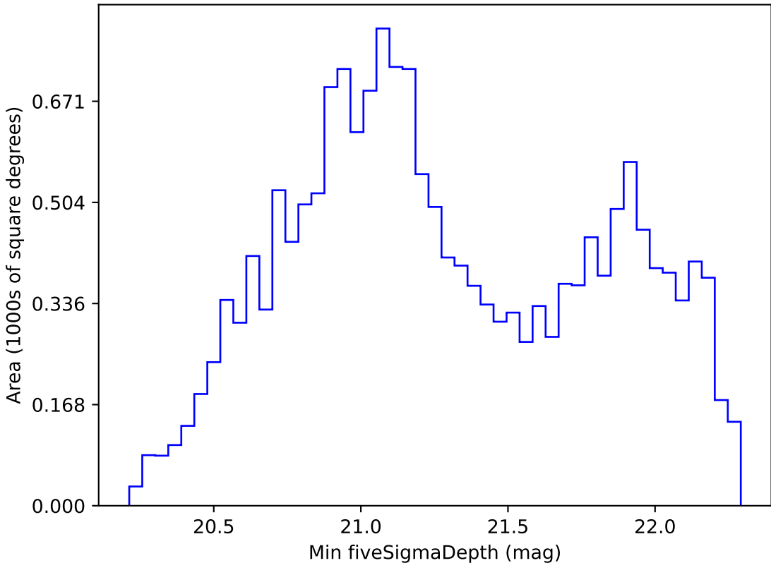
roll_pause_mjdp270_v3.4_10yrs WFD z band: Min fiveSigmaDepth
