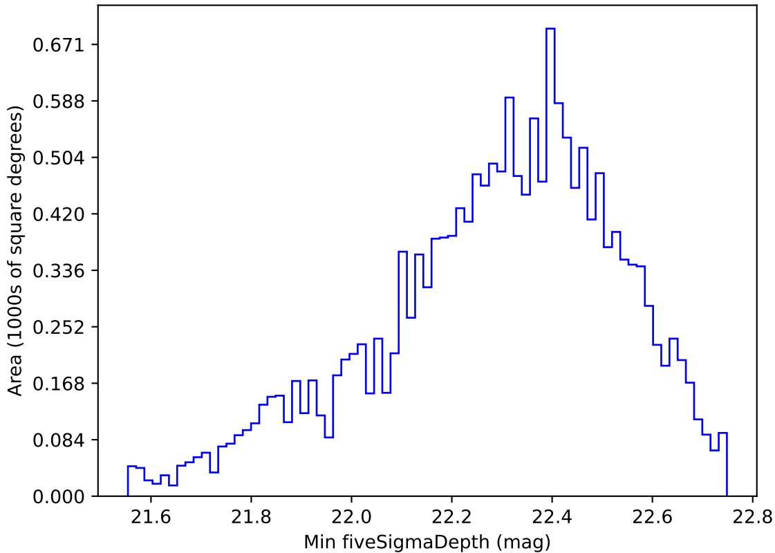
roll_pause_mjdp270_v3.4_10yrs WFD u band: Min fiveSigmaDepth
