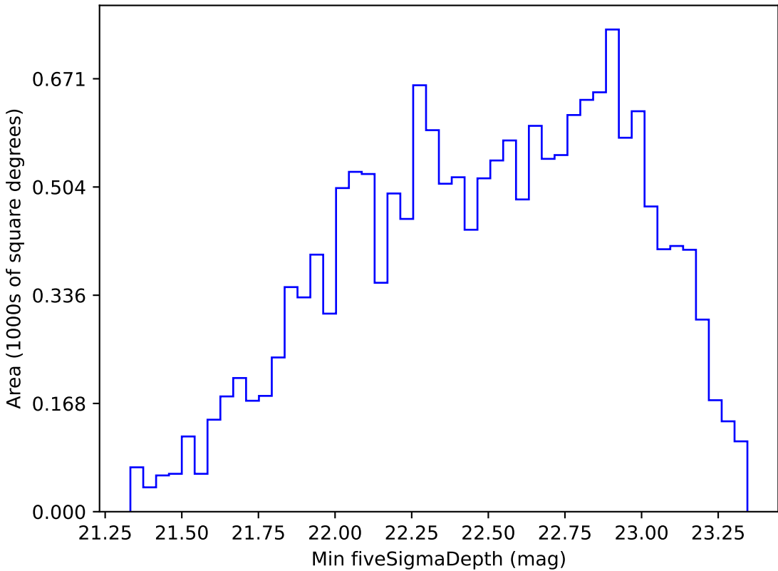
roll_pause_mjdp270_v3.4_10yrs WFD r band: Min fiveSigmaDepth
