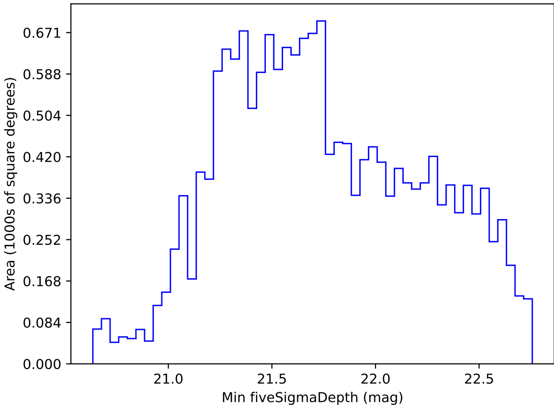
roll_pause_mjdp270_v3.4_10yrs WFD i band: Min fiveSigmaDepth
