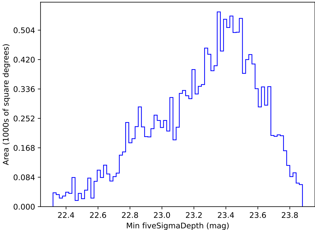
roll_pause_mjdp270_v3.4_10yrs WFD g band: Min fiveSigmaDepth
