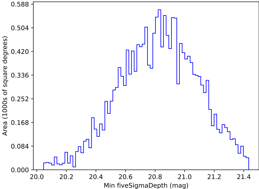
roll_pause_mjdp270_v3.4_10yrs WFD all bands: Min fiveSigmaDepth
