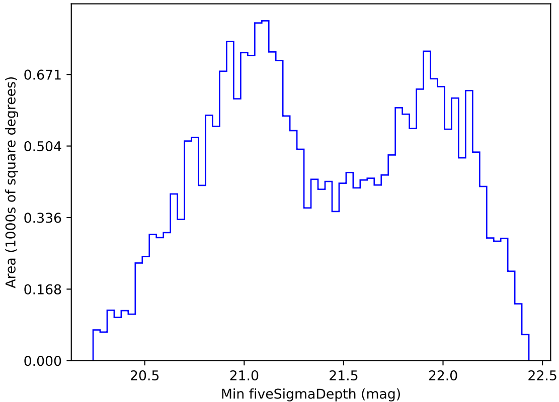
roll_pause_mjdp270_v3.4_10yrs All sky z band: Min fiveSigmaDepth
