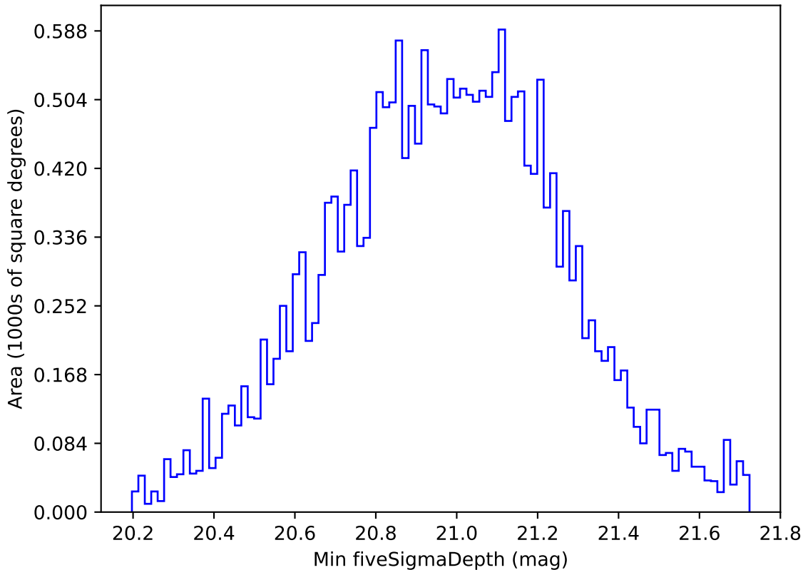
roll_pause_mjdp270_v3.4_10yrs All sky y band: Min fiveSigmaDepth
