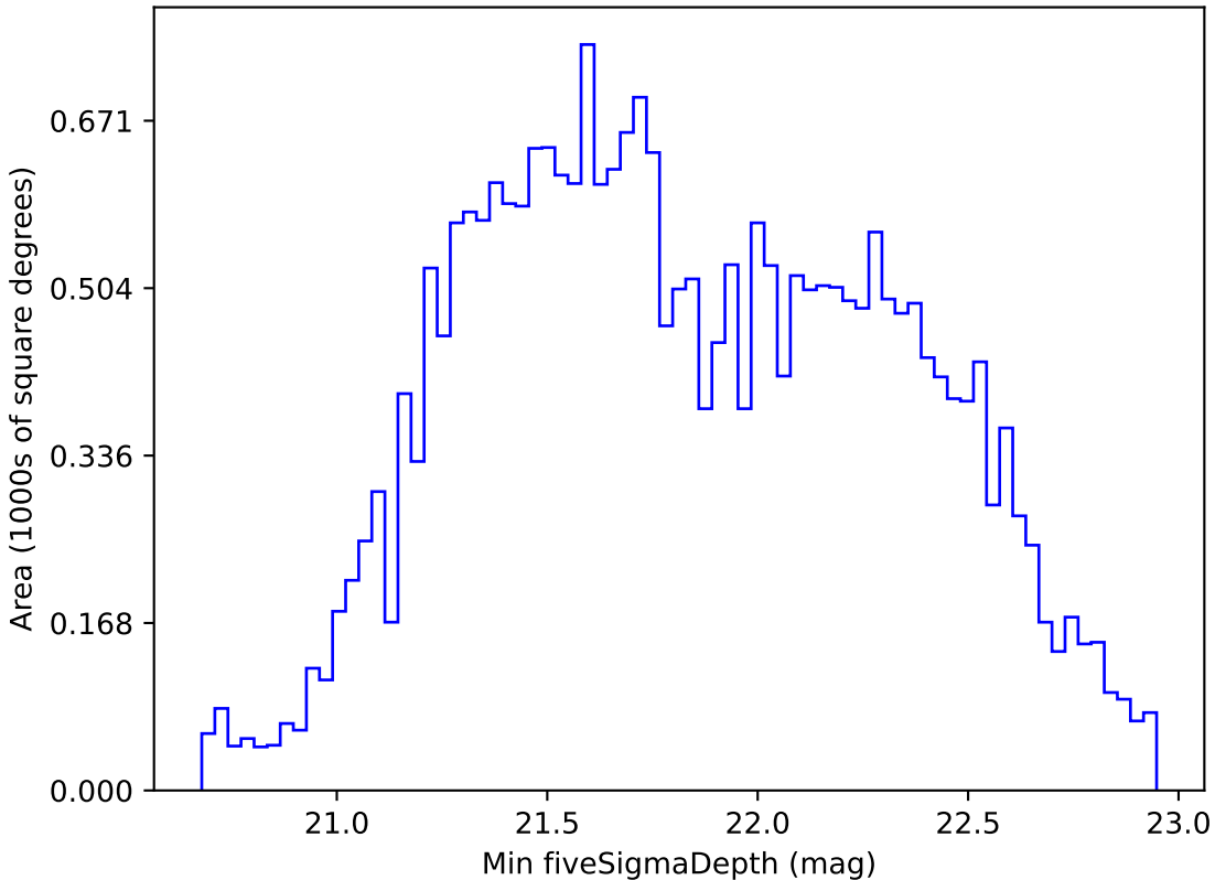
roll_pause_mjdp270_v3.4_10yrs All sky i band: Min fiveSigmaDepth
