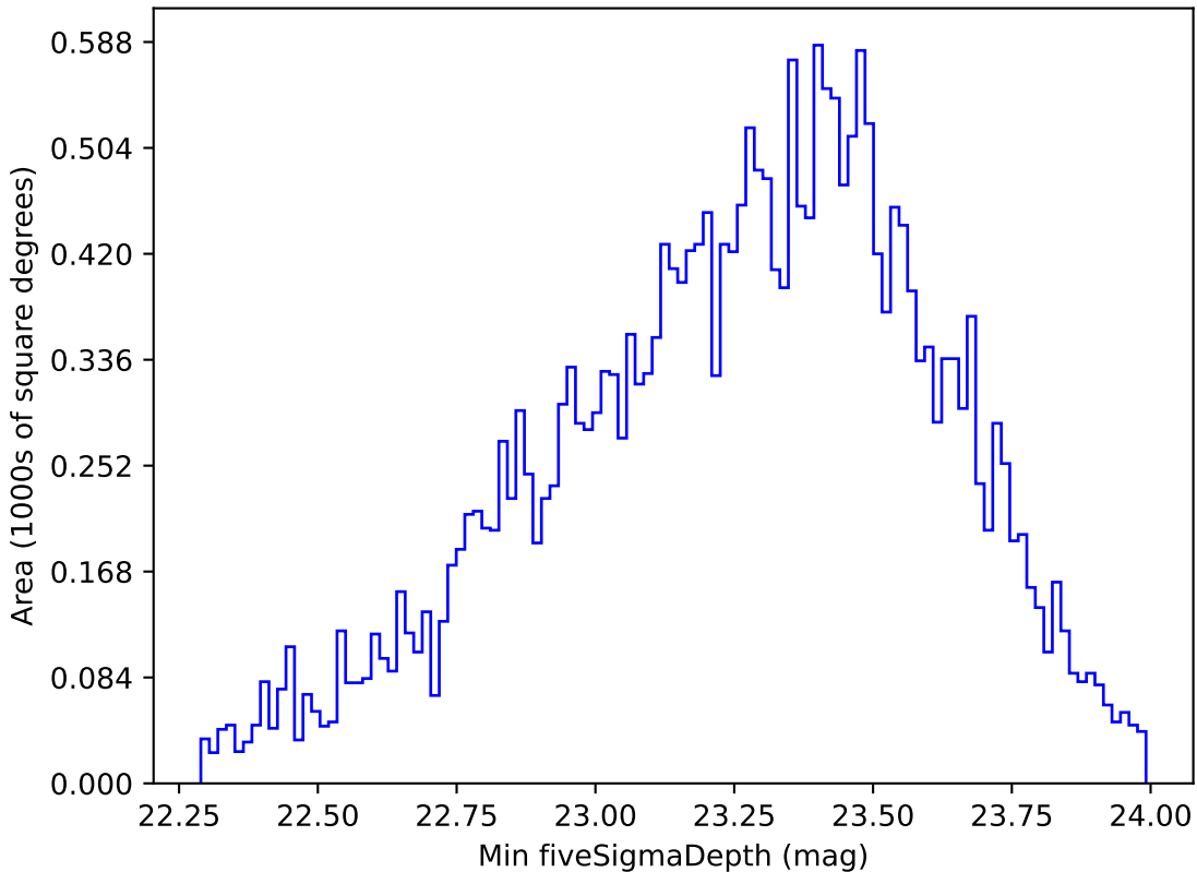
roll_pause_mjdp270_v3.4_10yrs All sky g band: Min fiveSigmaDepth
