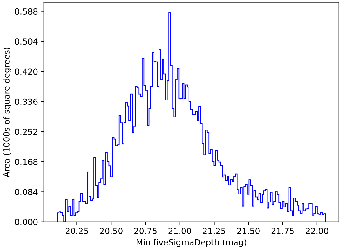
roll_pause_mjdp270_v3.4_10yrs All sky all bands: Min fiveSigmaDepth
