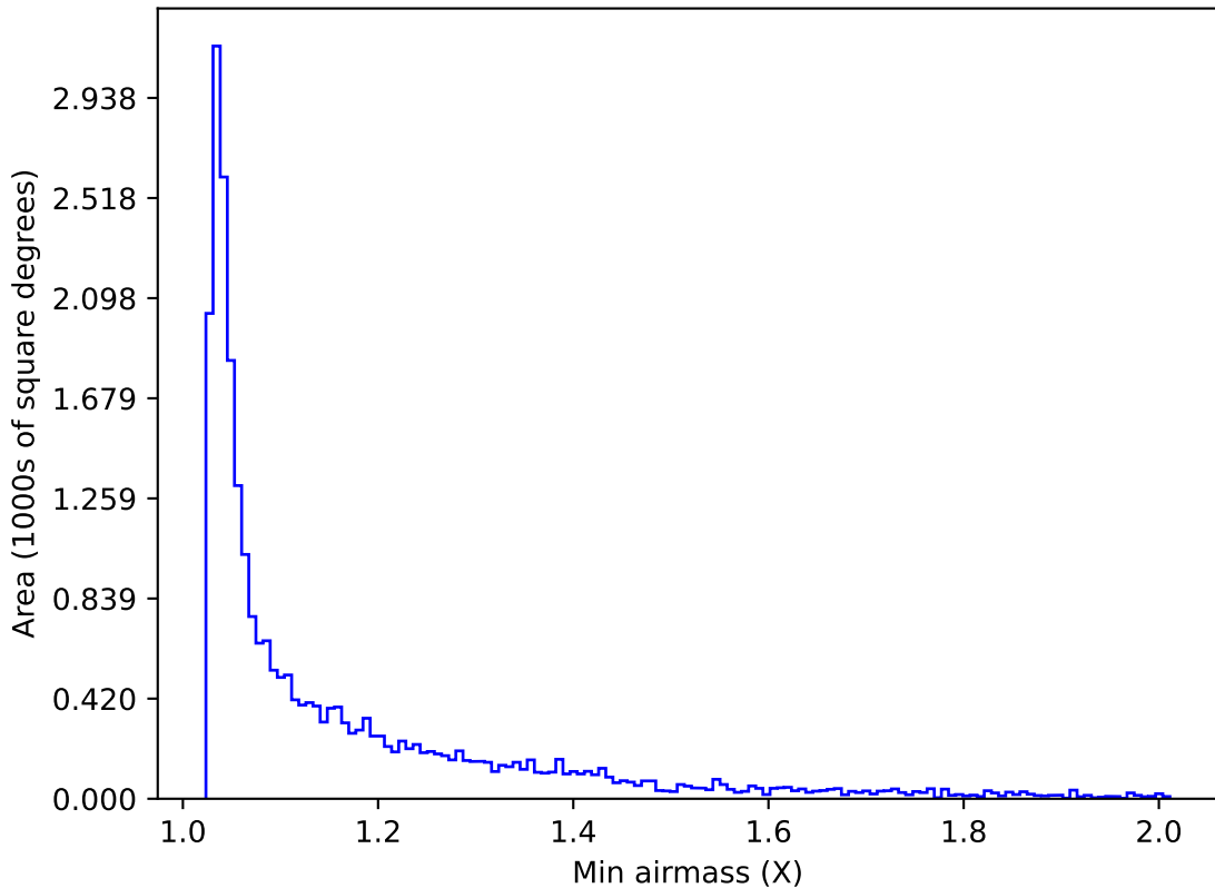
roll_pause_mjdp270_v3.4_10yrs Yr 1 r band: Min airmass
