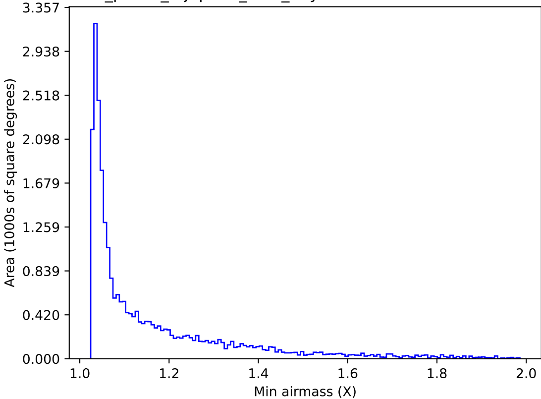
roll_pause_mjdp270_v3.4_10yrs Yr 1 i band: Min airmass
