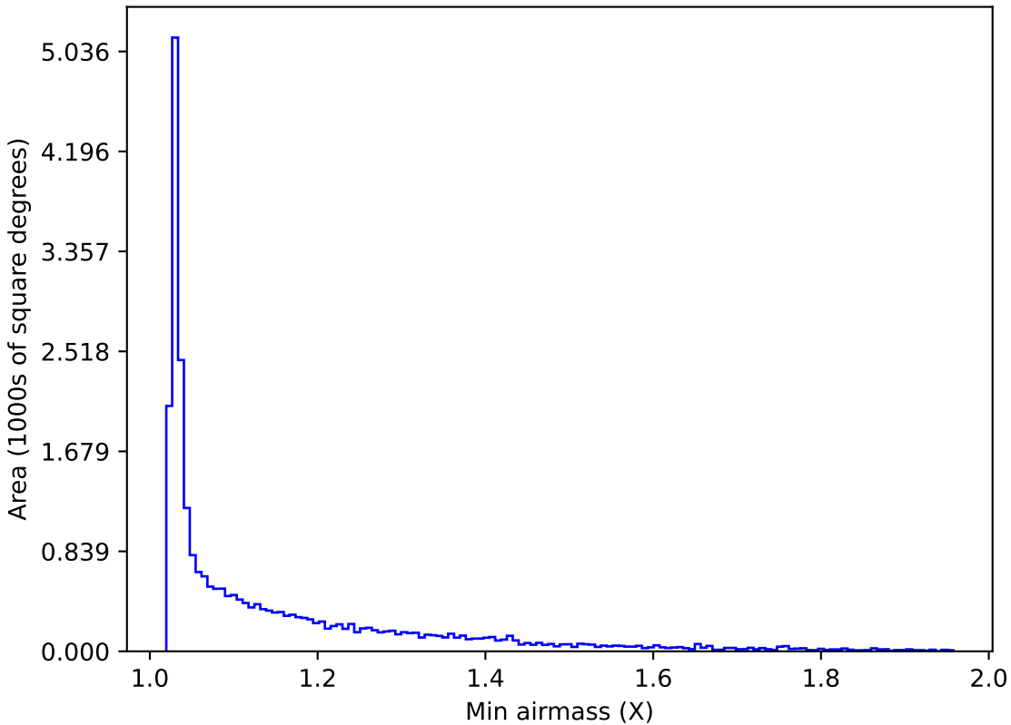
roll_pause_mjdp270_v3.4_10yrs Yr 1 all bands: Min airmass
