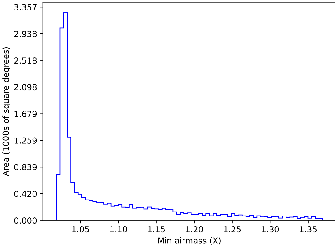
roll_pause_mjdp270_v3.4_10yrs WFD z band: Min airmass
