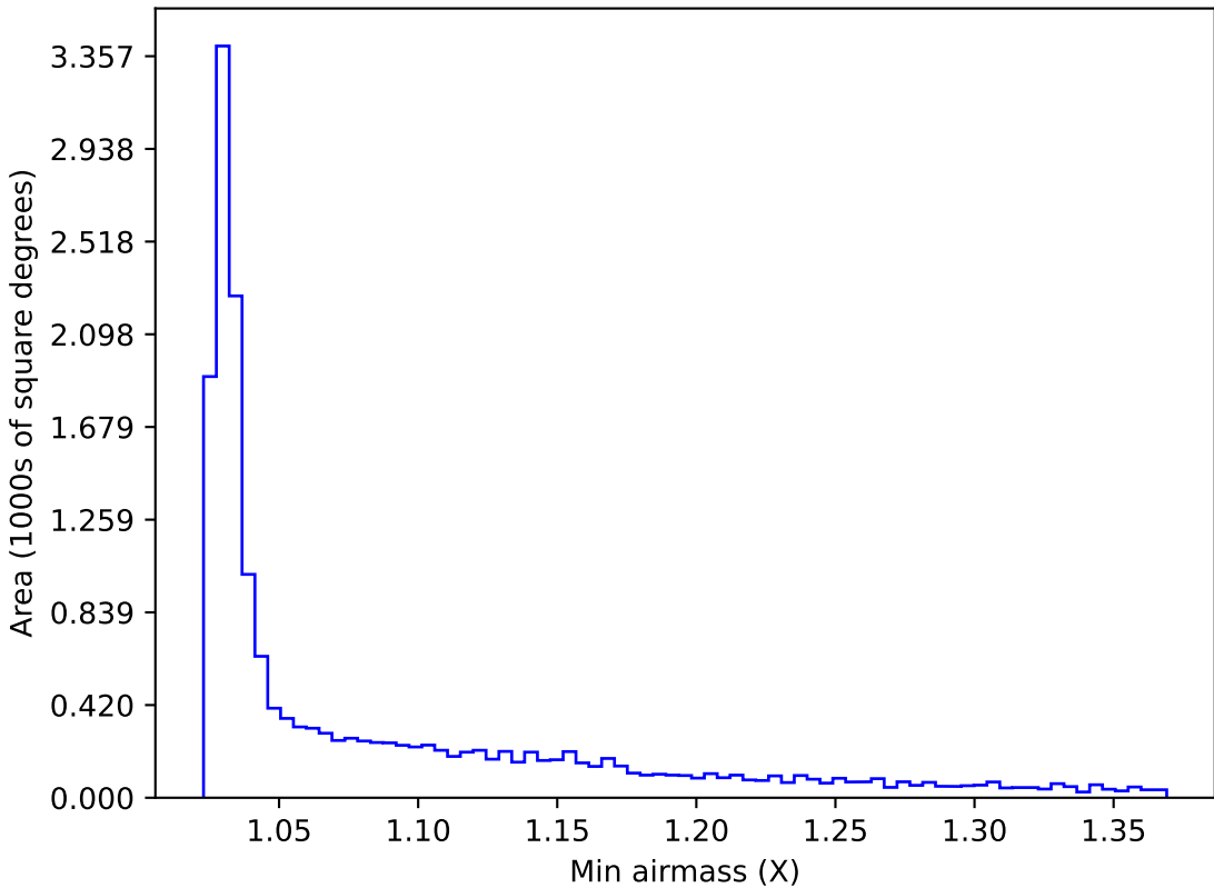
roll_pause_mjdp270_v3.4_10yrs WFD y band: Min airmass
