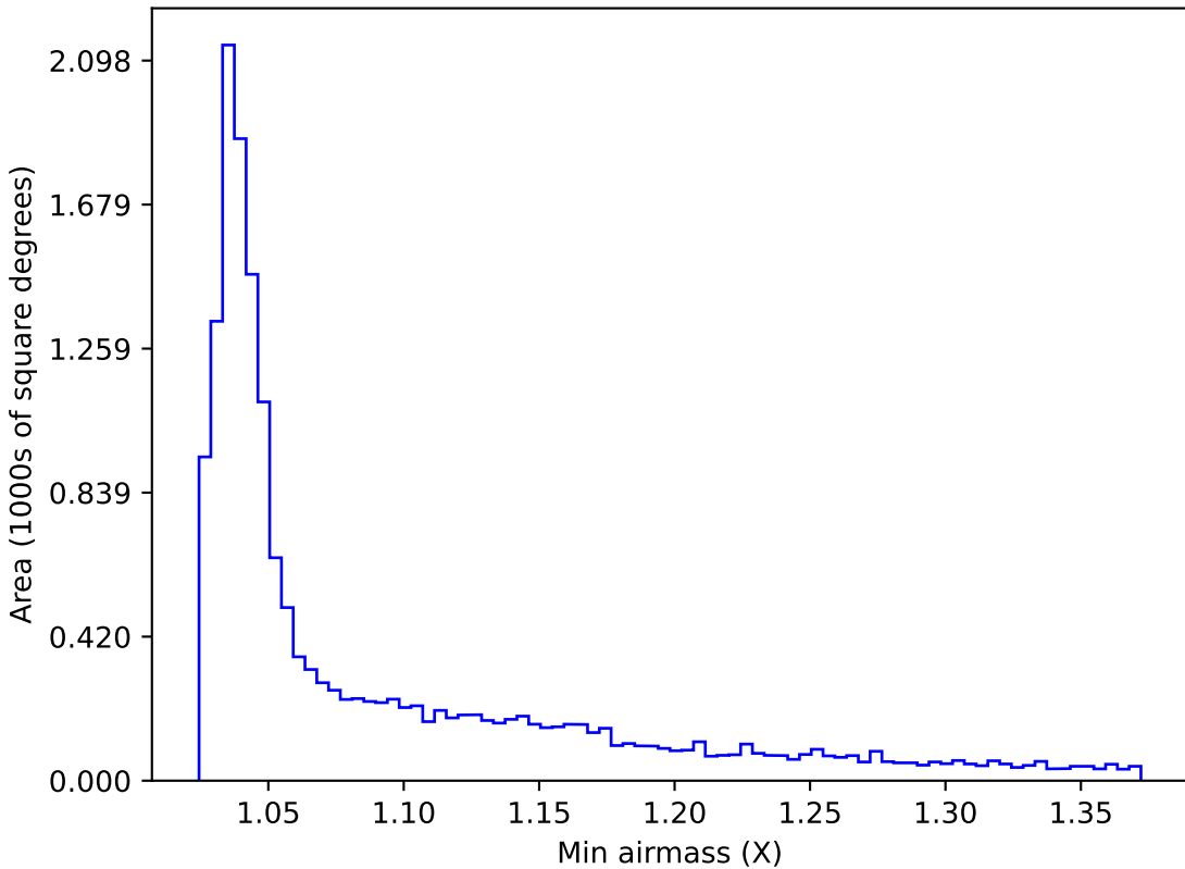
roll_pause_mjdp270_v3.4_10yrs WFD u band: Min airmass
