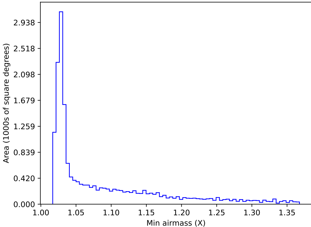
roll_pause_mjdp270_v3.4_10yrs WFD r band: Min airmass
