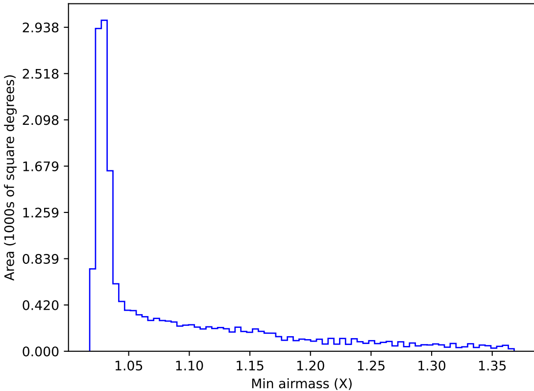
roll_pause_mjdp270_v3.4_10yrs WFD i band: Min airmass
