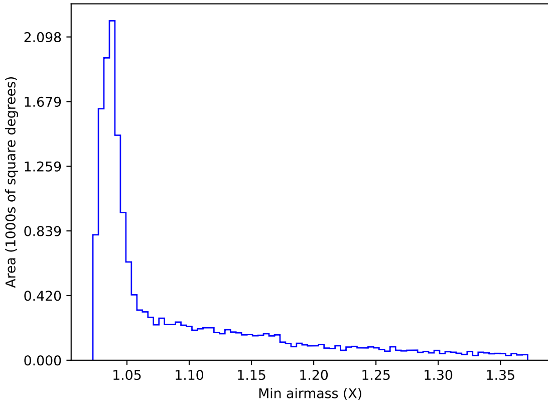
roll_pause_mjdp270_v3.4_10yrs WFD g band: Min airmass
