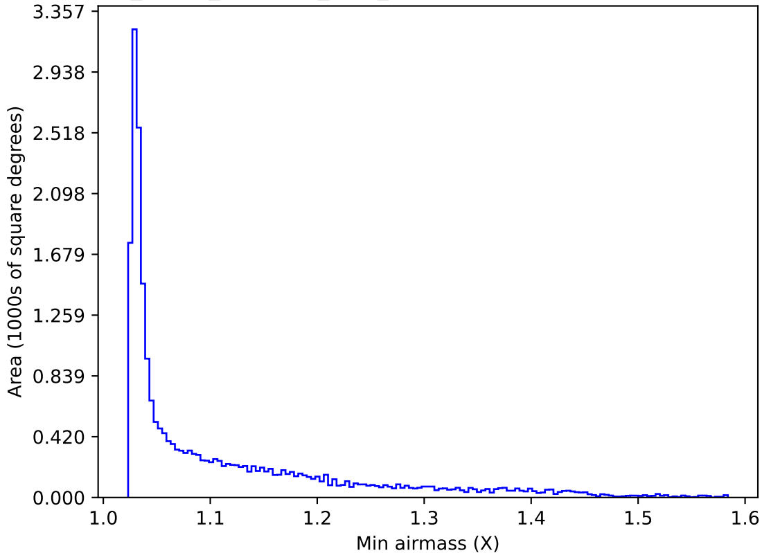
roll_pause_mjdp270_v3.4_10yrs All sky y band: Min airmass
