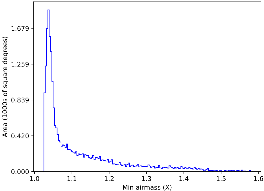
roll_pause_mjdp270_v3.4_10yrs All sky u band: Min airmass
