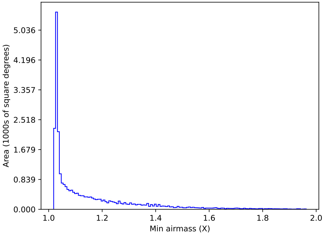
roll_pause_mjdp270_v3.4_10yrs All sky i band: Min airmass
