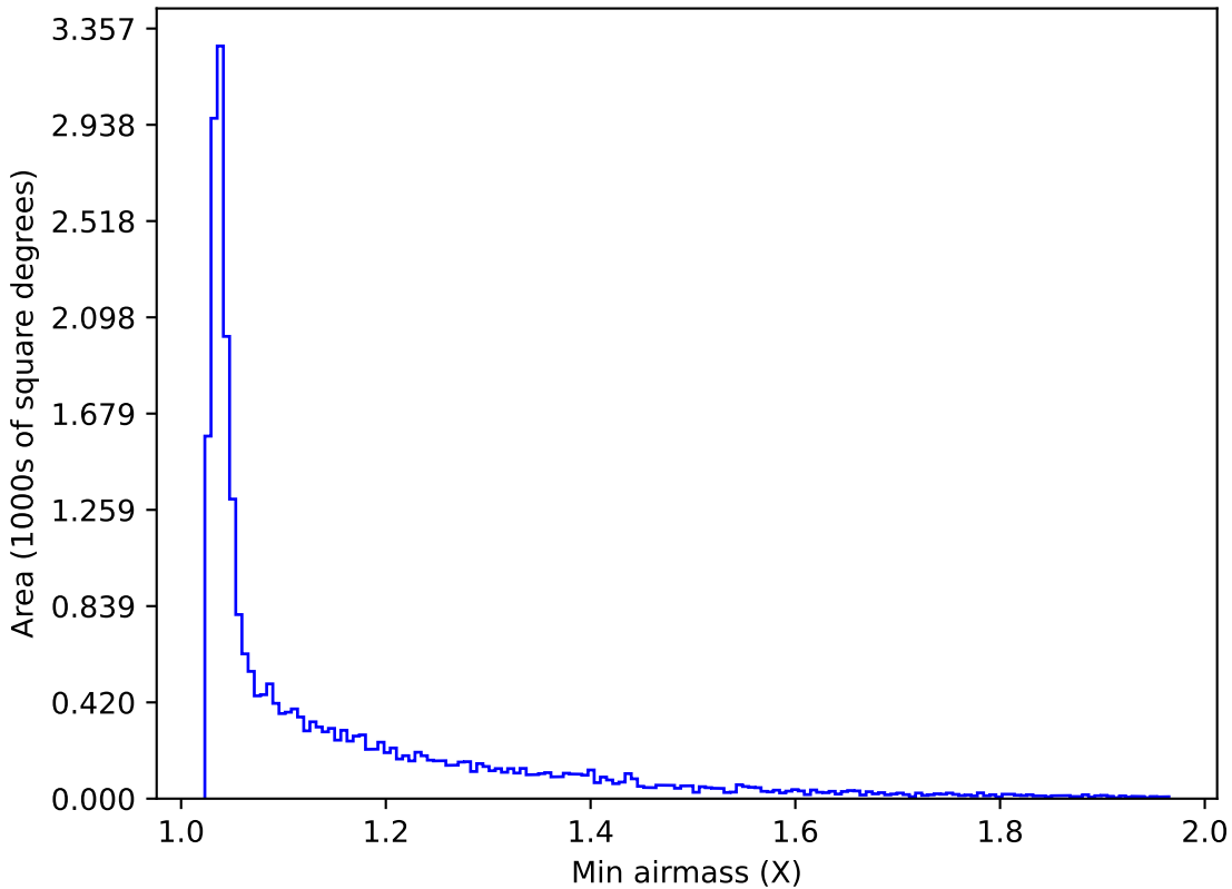
roll_pause_mjdp270_v3.4_10yrs All sky g band: Min airmass
