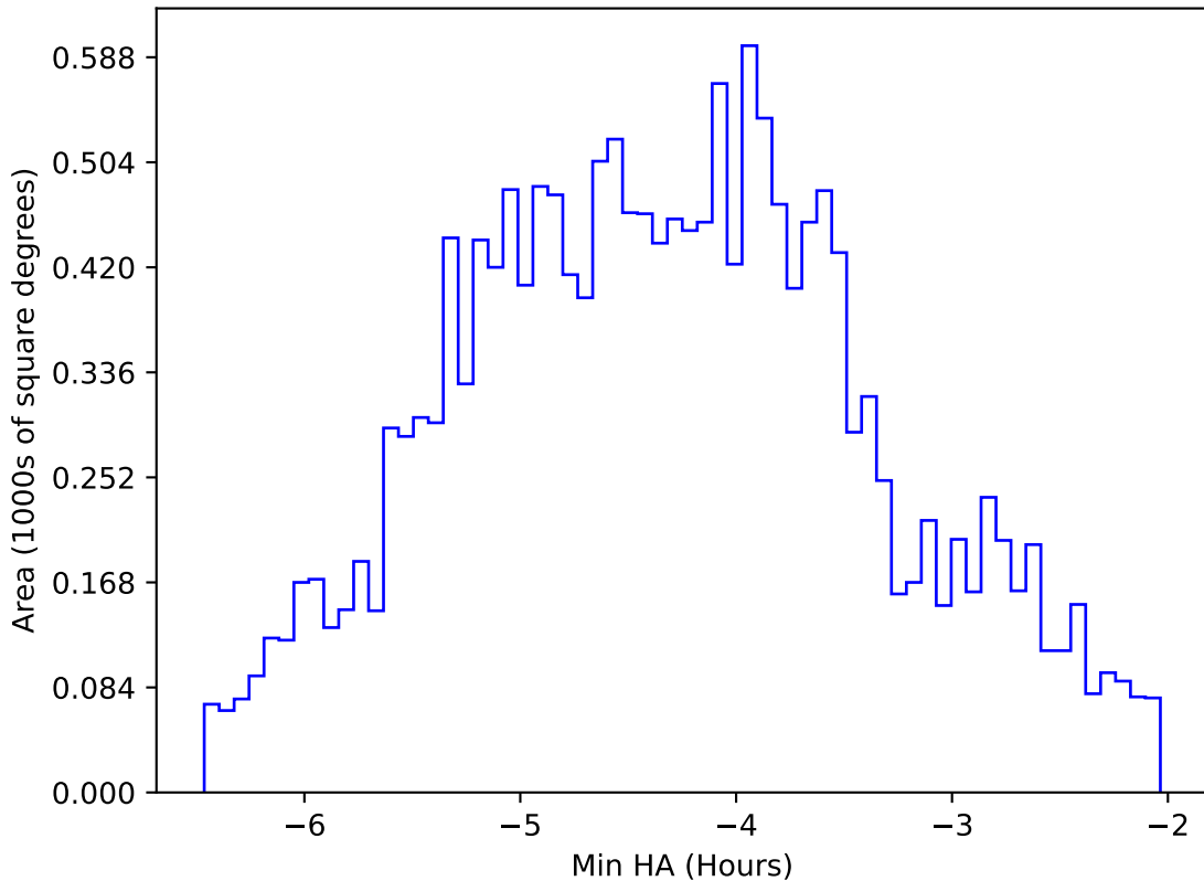
roll_pause_mjdp270_v3.4_10yrs WFD z band: Min HA
