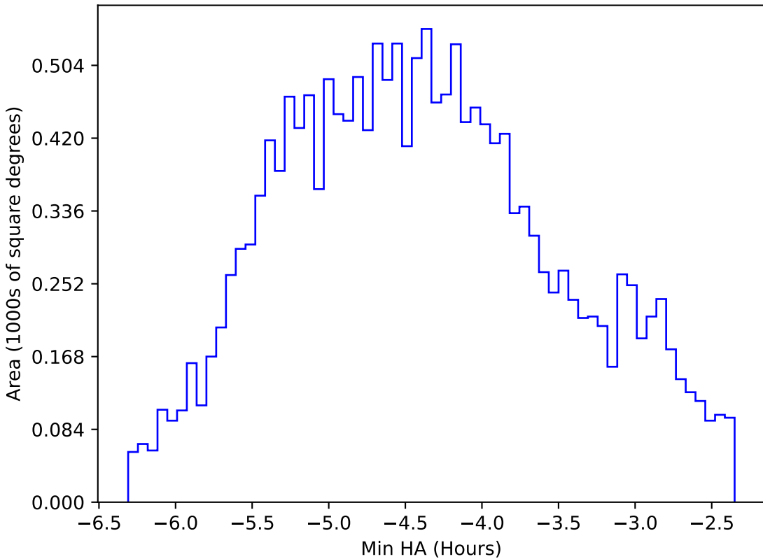
roll_pause_mjdp270_v3.4_10yrs WFD r band: Min HA
