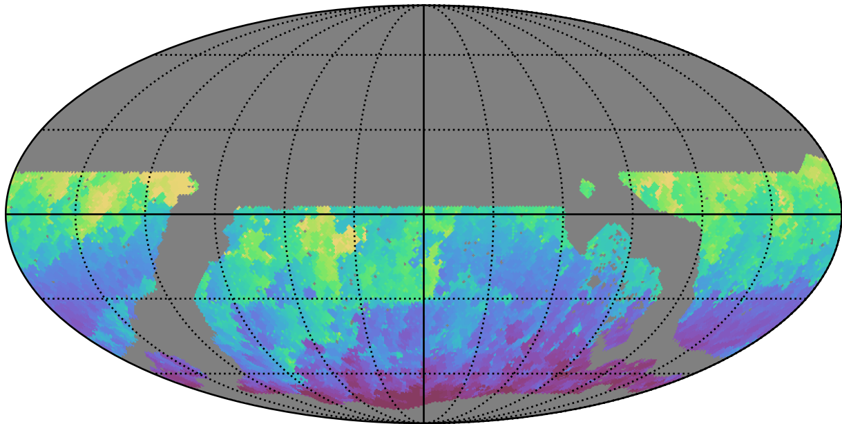
roll_pause_mjdp270_v3.4_10yrs WFD i band: Min HA
