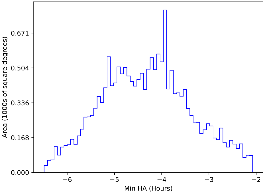
roll_pause_mjdp270_v3.4_10yrs WFD i band: Min HA
