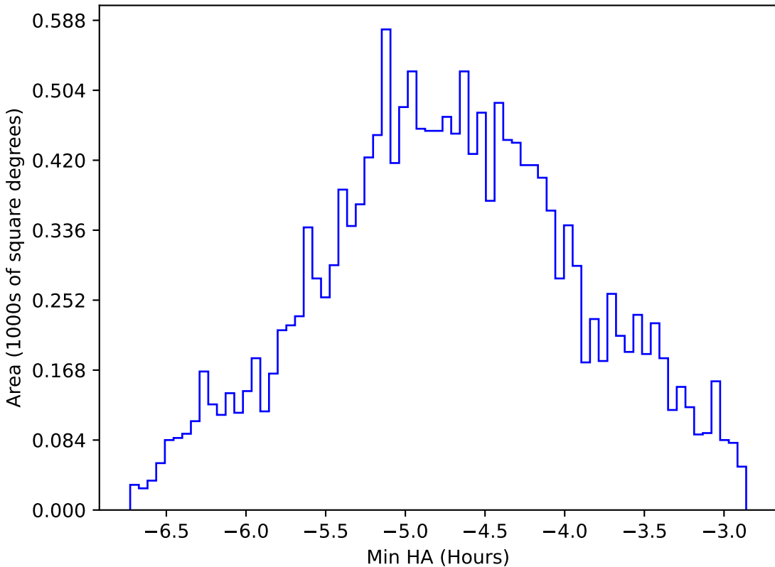
roll_pause_mjdp270_v3.4_10yrs WFD all bands: Min HA
