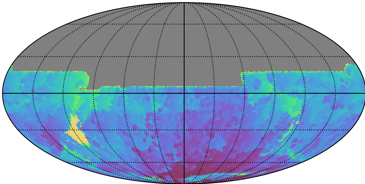
roll_pause_mjdp270_v3.4_10yrs All sky y band: Min HA
