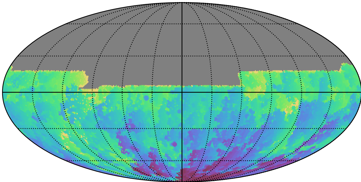
roll_pause_mjdp270_v3.4_10yrs All sky u band: Min HA
