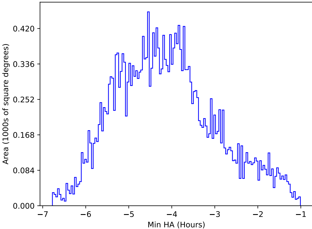
roll_pause_mjdp270_v3.4_10yrs All sky r band: Min HA
