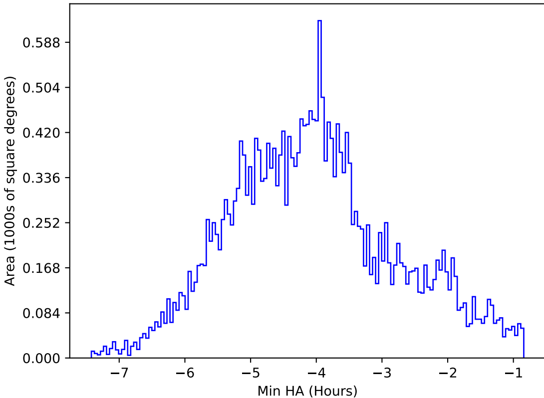
roll_pause_mjdp270_v3.4_10yrs All sky i band: Min HA
