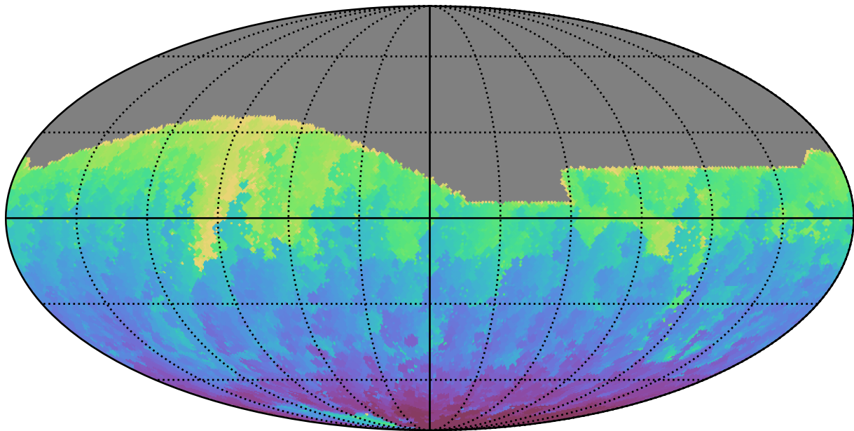
roll_pause_mjdp270_v3.4_10yrs All sky g band: Min HA
