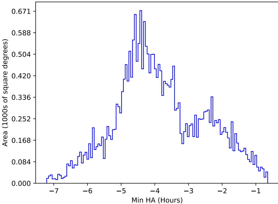
roll_pause_mjdp270_v3.4_10yrs All sky g band: Min HA
