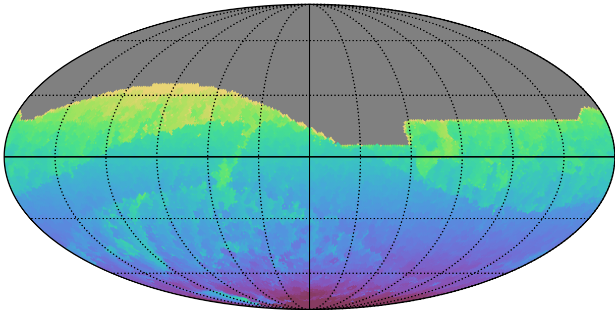
roll_pause_mjdp270_v3.4_10yrs All sky all bands: Min HA
