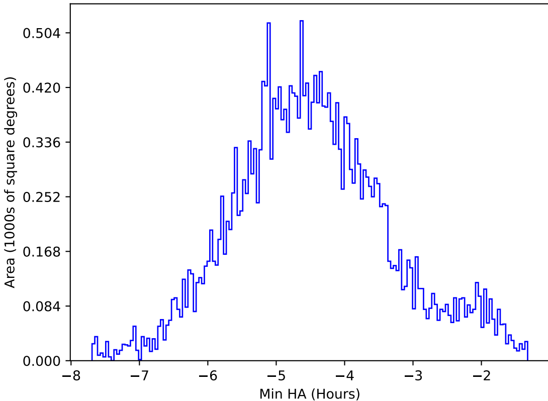
roll_pause_mjdp270_v3.4_10yrs All sky all bands: Min HA
