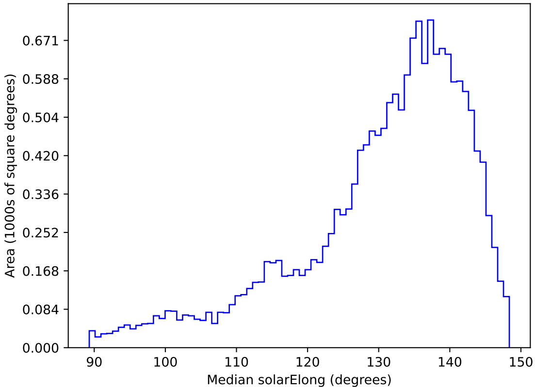
roll_pause_mjdp270_v3.4_10yrs WFD y band: Median solarElong
