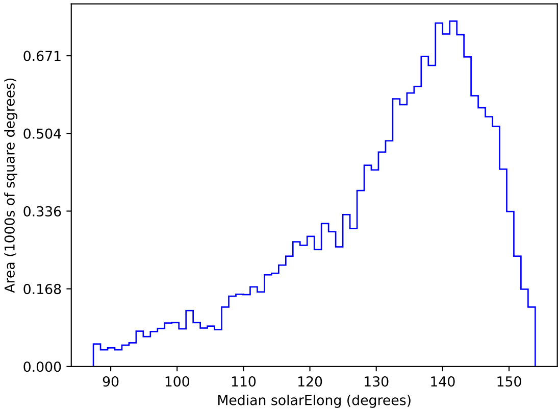
roll_pause_mjdp270_v3.4_10yrs WFD u band: Median solarElong
