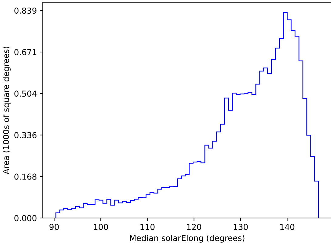
roll_pause_mjdp270_v3.4_10yrs WFD r band: Median solarElong
