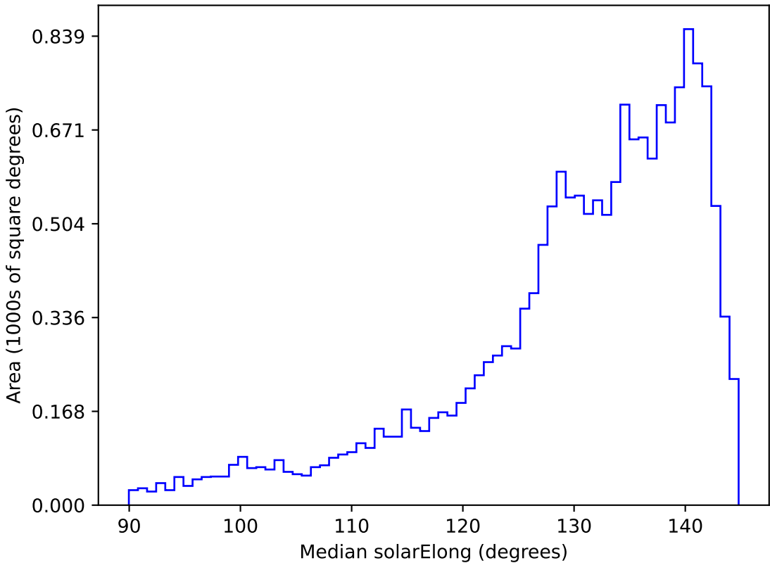
roll_pause_mjdp270_v3.4_10yrs WFD all bands: Median solarElong
