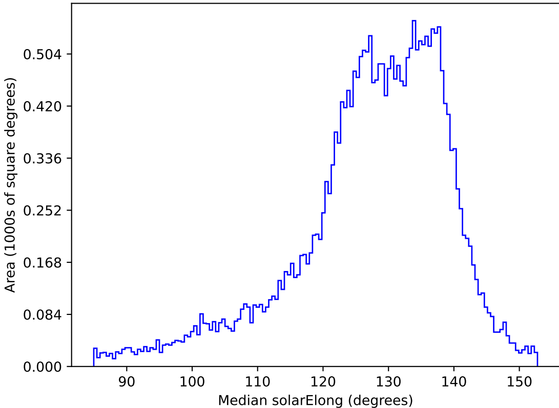
roll_pause_mjdp270_v3.4_10yrs All sky z band: Median solarElong
