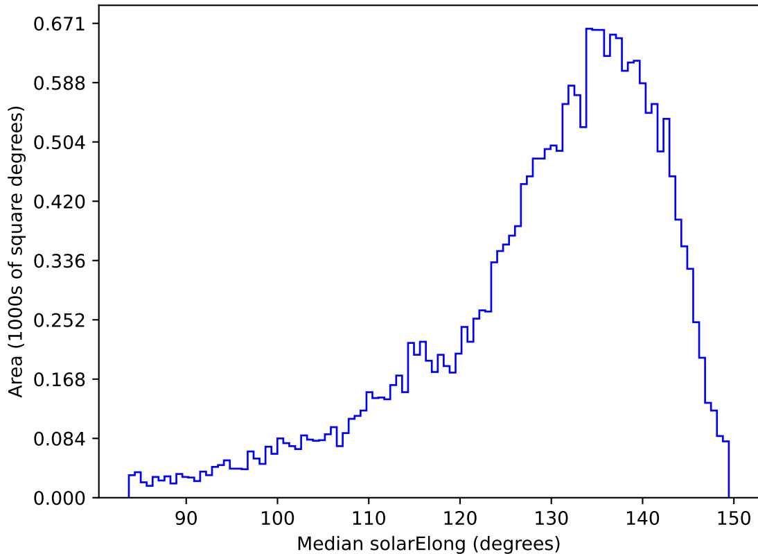
roll_pause_mjdp270_v3.4_10yrs All sky y band: Median solarElong
