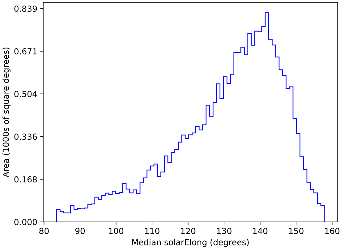
roll_pause_mjdp270_v3.4_10yrs All sky u band: Median solarElong
